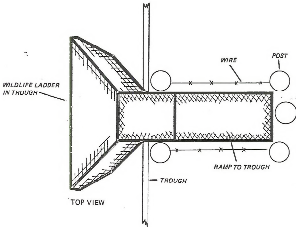
ILLUSTRATION 5: Fencing and post arrangement to protect wildlife ramp leading into a livestock watering facility.
